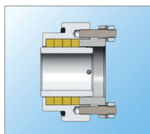
Gland packing
