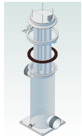
Magnetic filter FMF 420/6
